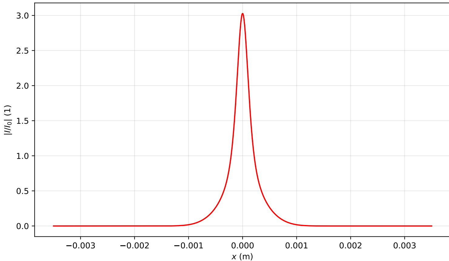
Intensity profile I(x, y = 0, z = 0.478)/I_0 , P_{in}=3.5P_{cr} , artificial time
